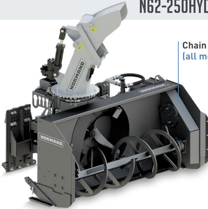
N62-250HYD Without backdrag (scraper blade)
